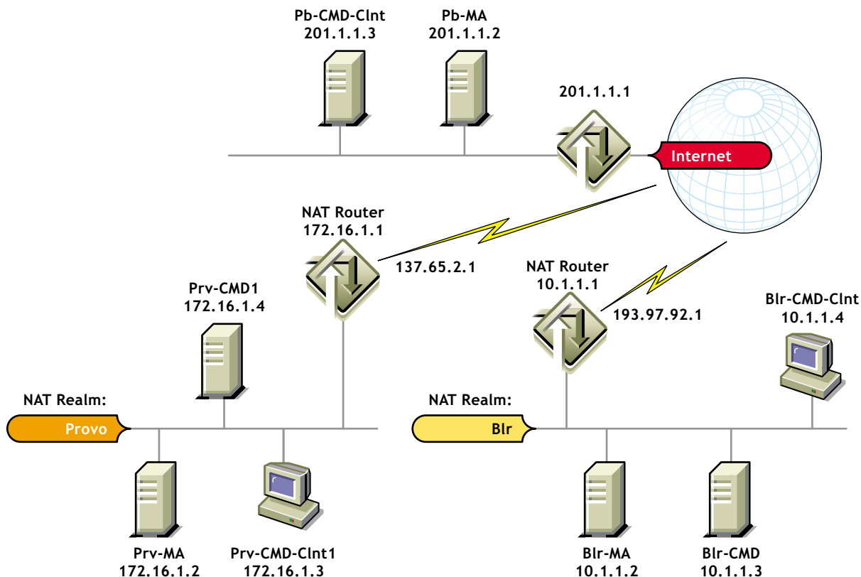
Figure 16 Two private routing realms, BLR and Provo, connected by a public realm to the Internet
