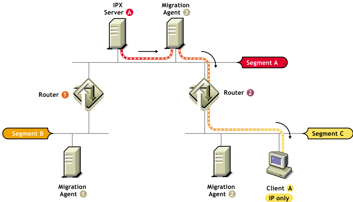
Figure 13 Sample Network Setup for Example 1
