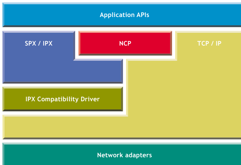
Figure 5 IP Only Architecture Diagram
