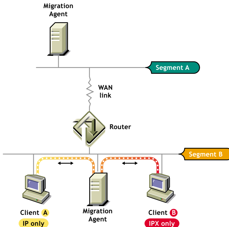
Figure 15 Sample Network Setup for Example 2
